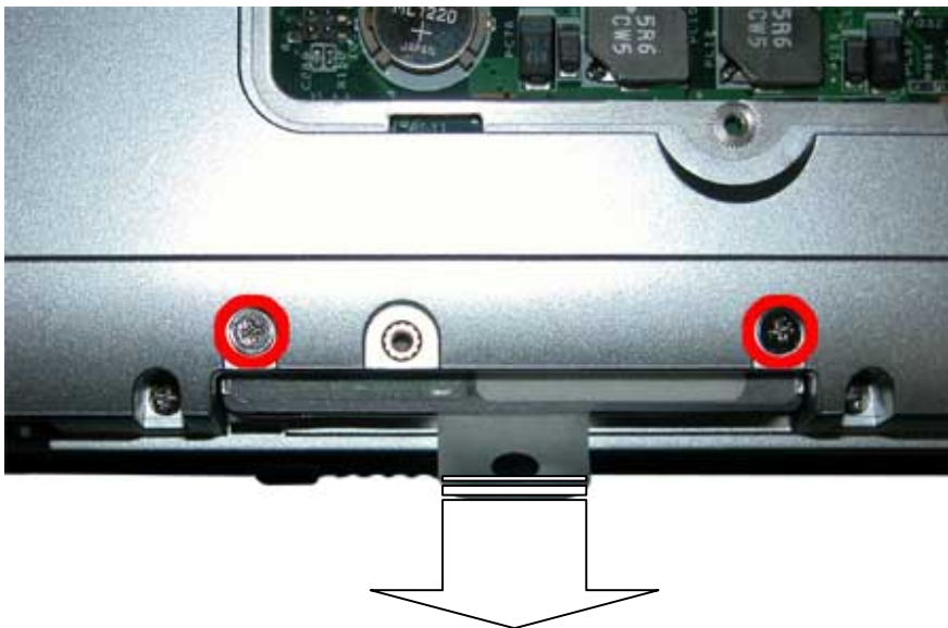
Fig. 6 Screw retaining the HDD module
